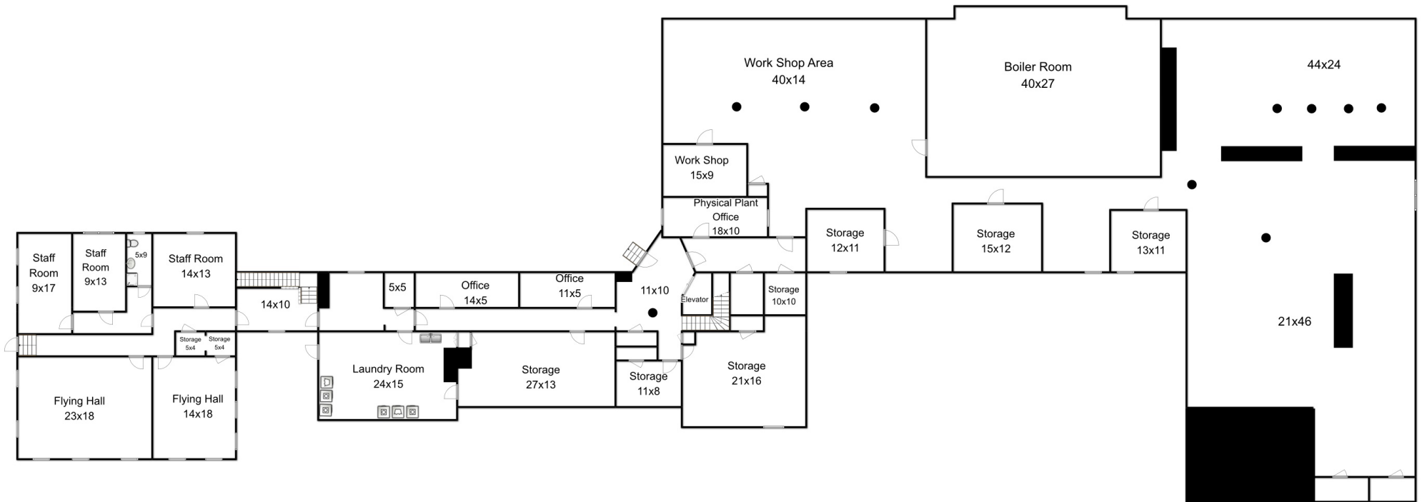
Main House: Lower Floor
