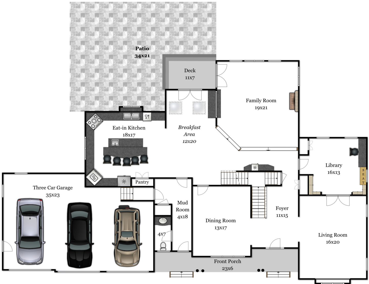
First Floor
