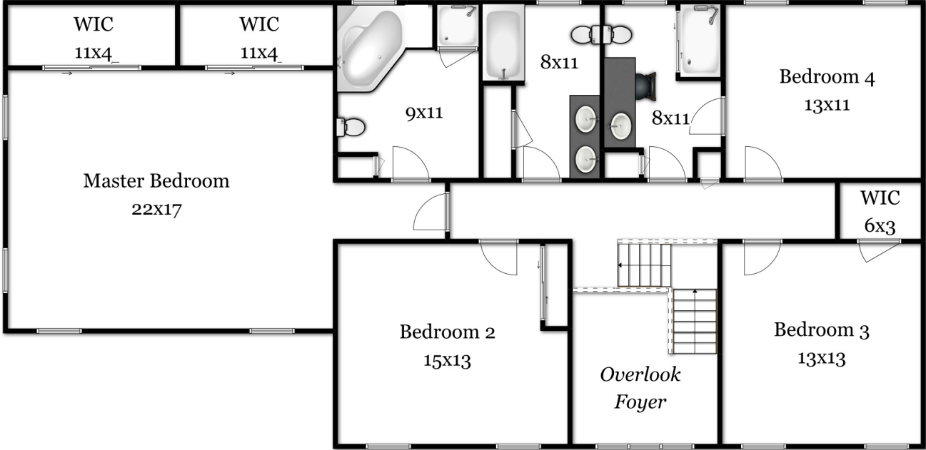
Second Floor
