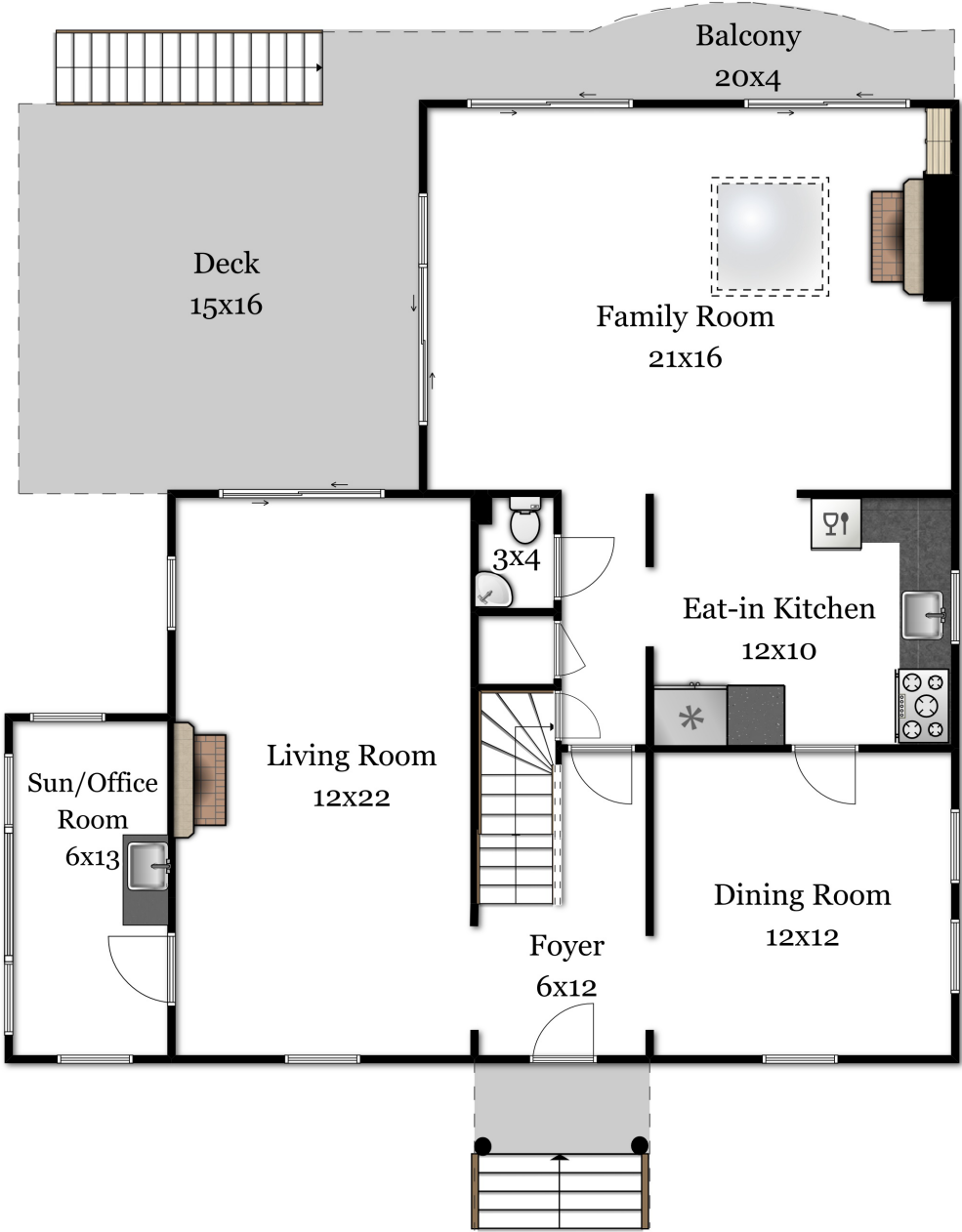
First Floor
