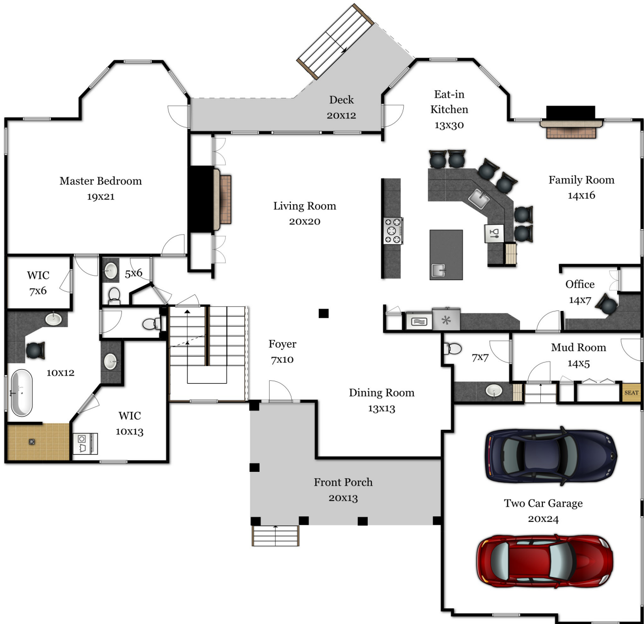
First Floor
