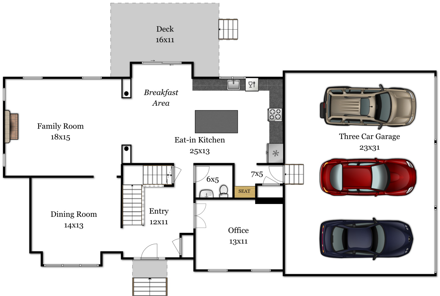
First Floor
