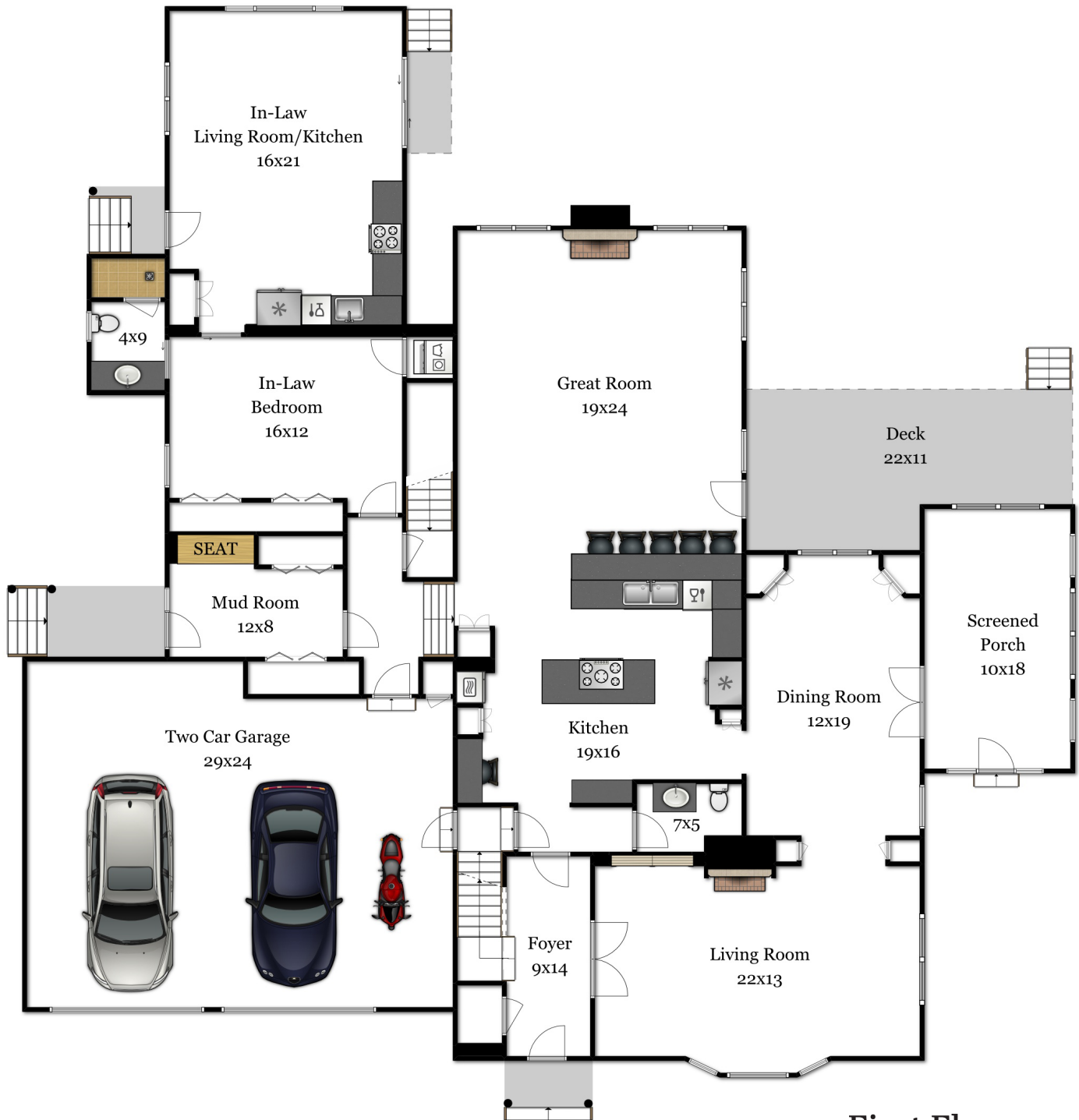
First Floor
