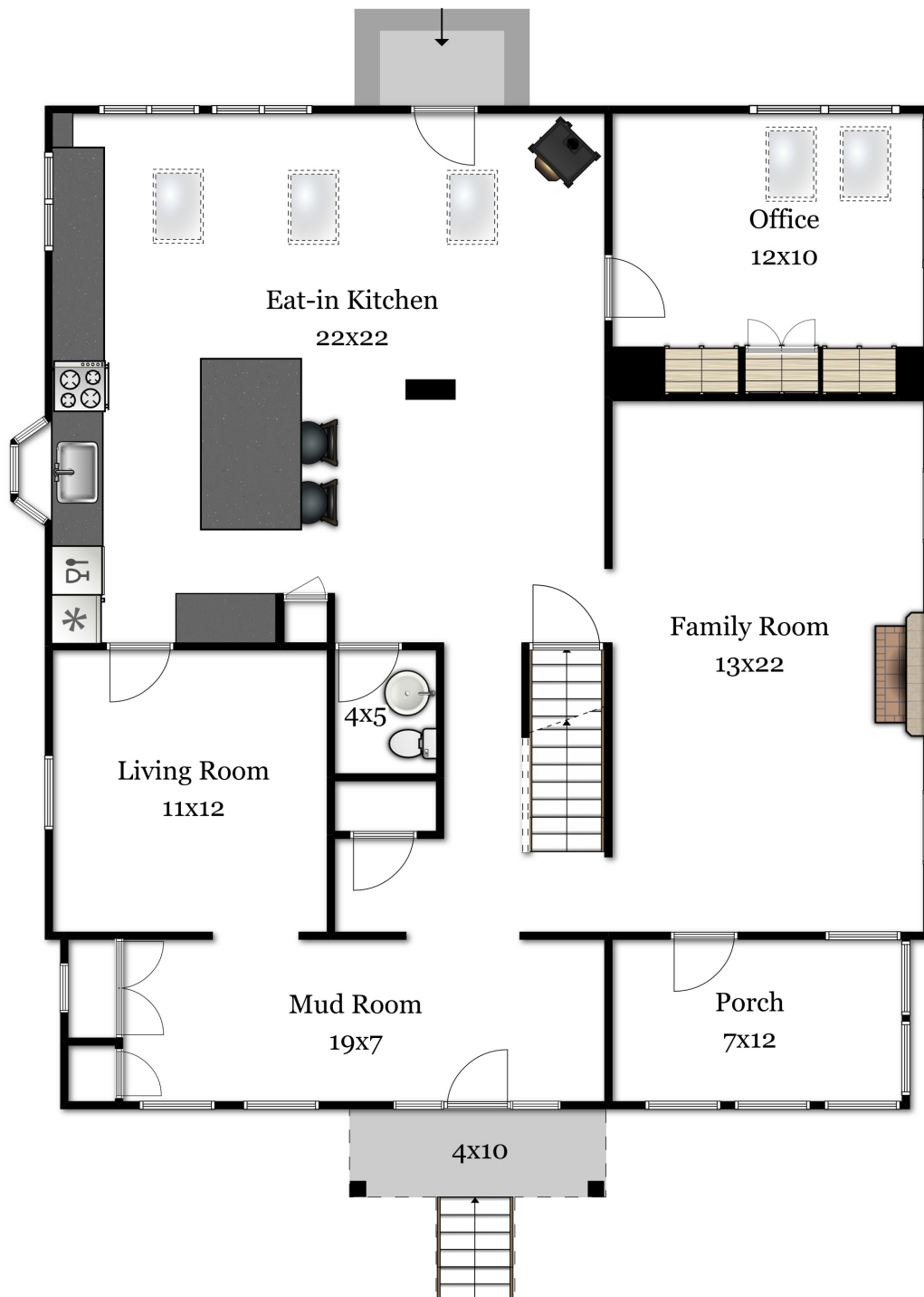
First Floor
