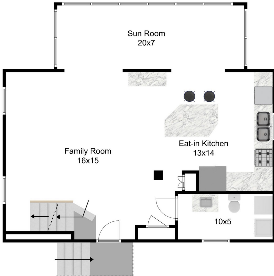
First Floor
